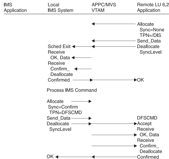
Figure 38. Flow of a Local IMS Asynchronous Command When Sync_level=Confirm
