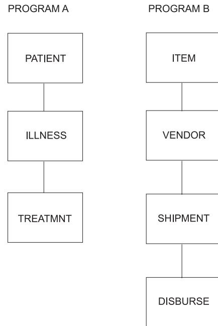
Figure 23. Patient and Inventory Hierarchies
