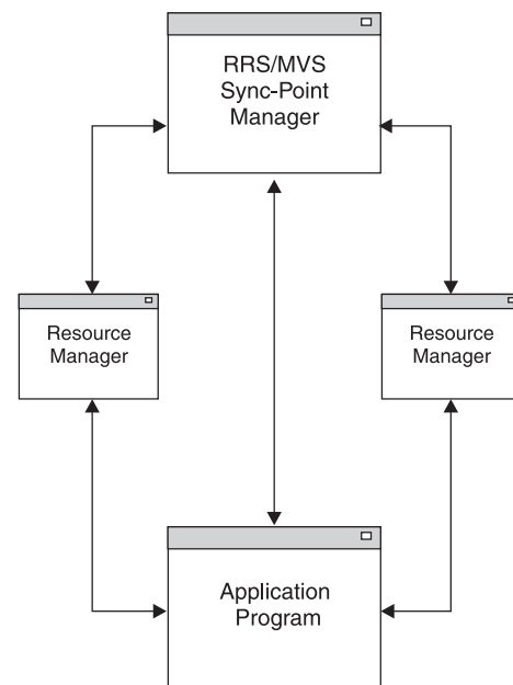
Figure 29. Participants in Resource Recovery
