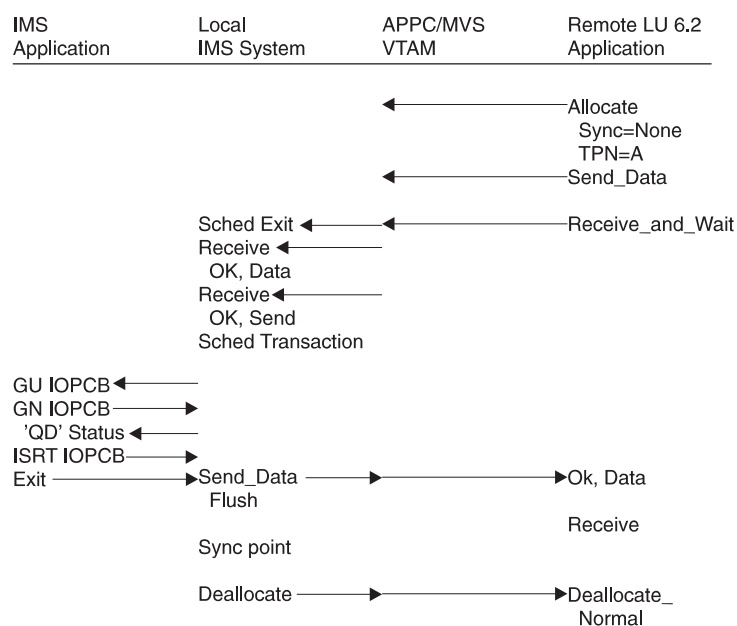
Figure 32. Flow of a Local IMS Synchronous Transaction When Sync_level=None
