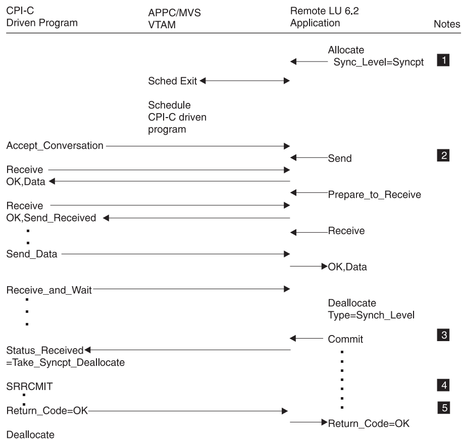
Figure 46. CPI-C Driven Commit Scenario When Sync_Level=Syncpt
