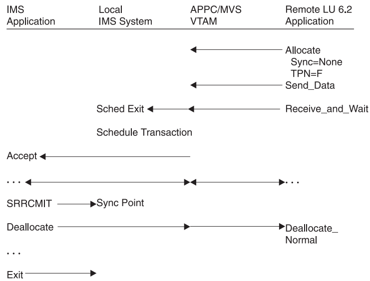
Figure 40. Flow of a Local CPI Communications Driven Program When Sync_level=None
