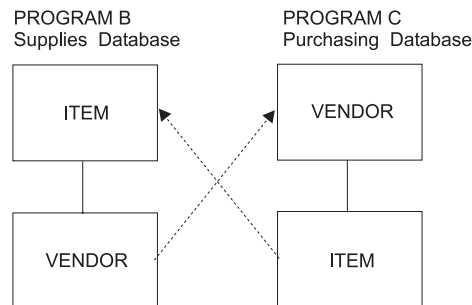
Figure 26. Program B and Program C Hierarchies
