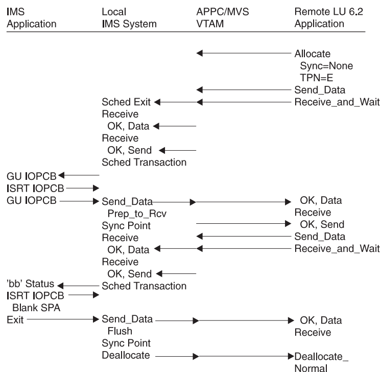
Figure 36. Flow of a Local IMS Conversational Transaction When Sync_level=None
